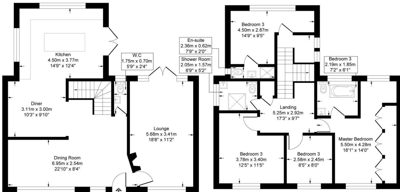
Ground Floor
